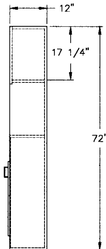
SIDE VIEW LESS SHAMPOO BOWLS
