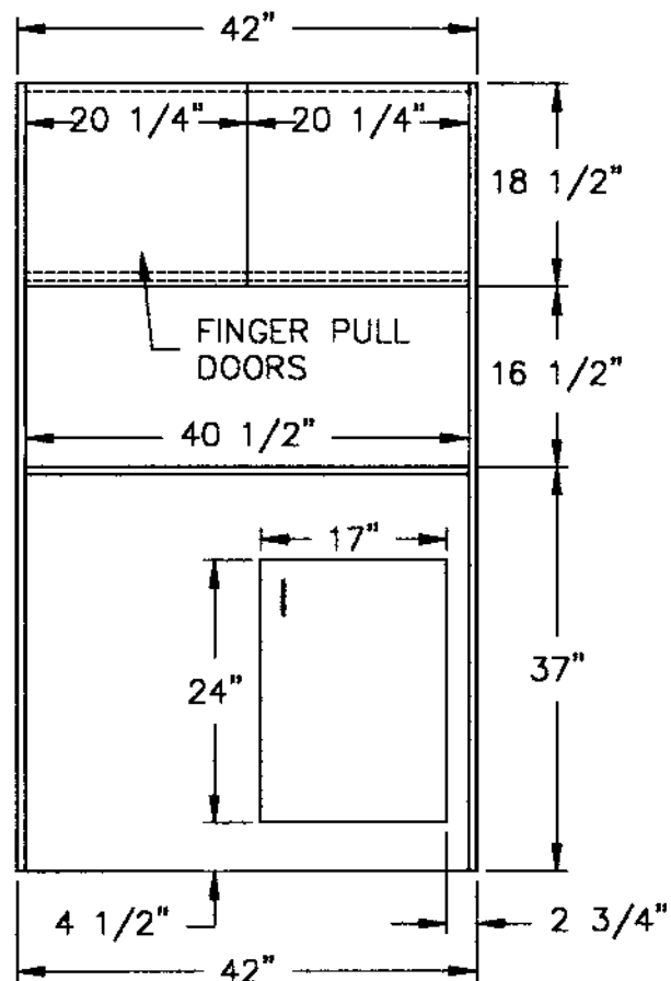
FRONT VIEW LESS SHAMPOO BOWLS
