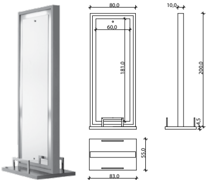
LIGHT MI/180
