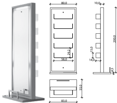
LIGHT MI/181
